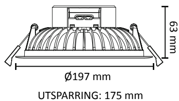
LED Compact 176
