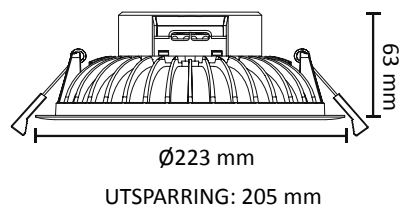
LED Compact 202
