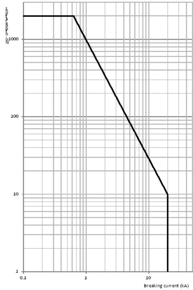
SafePlus V20 12, 15, 17,5 and 24 kV VG5
