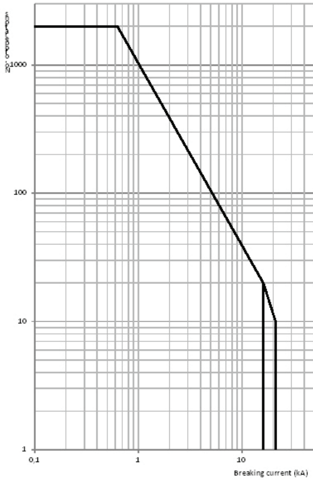
SafePlus V-module 12, 15, 17,5 and 24 kV
