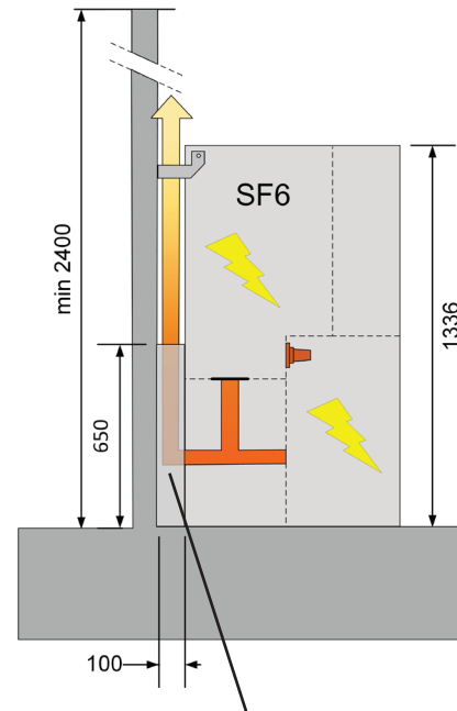
Arc shield Height of arc shield for M-module is 1317 mm.
