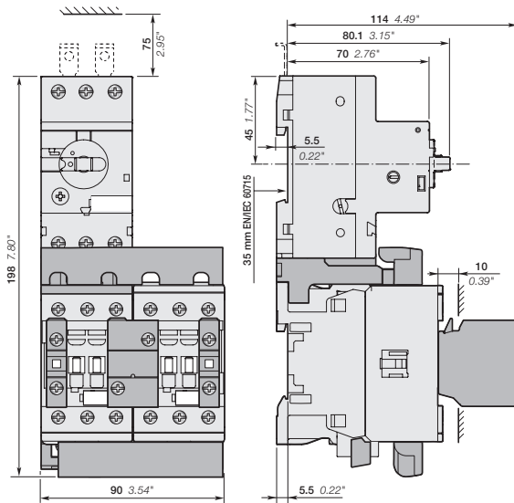
MS116 + BEA26-4, BER38-4, VEM4, CA4-10 + AF26, AF30, AF38
