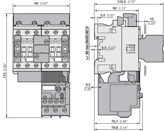
AF26, AF30, AF38 + BER38-4, VEM4, CA4-10 + TF42
