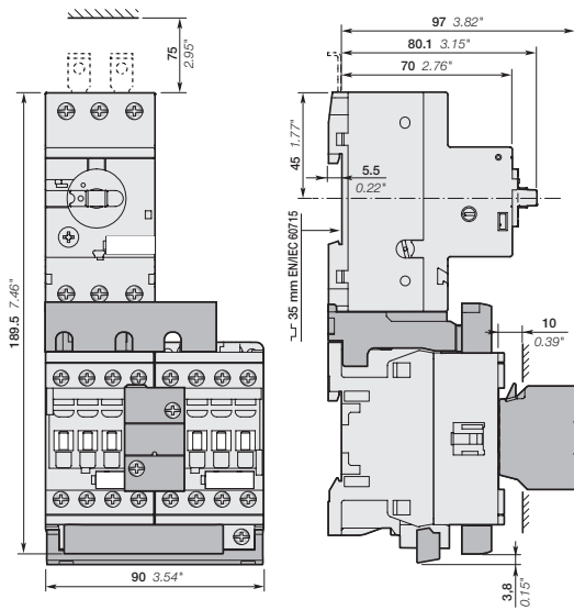
MS116 + BEA16-4, BER16-4, VEM4 + AF09, AF12, AF16
